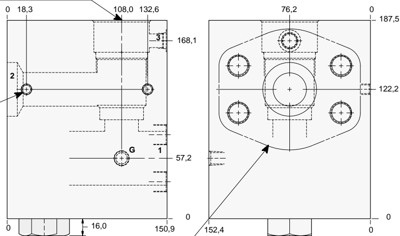
2.00" SAE Code 62 4-Bolt Flange Pattern 2 places.
